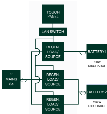
FIGURE 1 Independent testing of 2 different battery types
