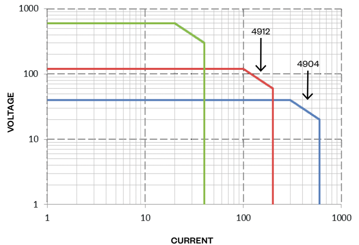
FIGURE 2 Discharge Operating Envelope
