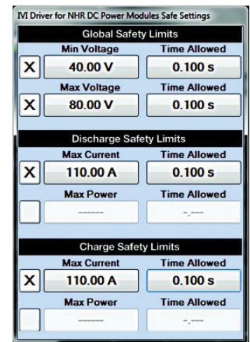
FIGURE 6 Safety Settings
